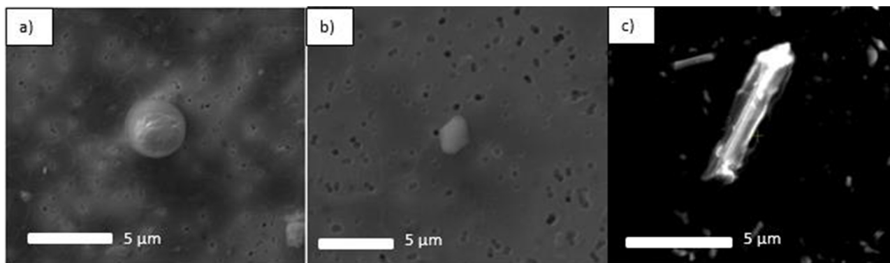
Fig. 9. Different inclusion morphology after dissolution. a) \text{SiO}_2 ; b) \text{SiO}_2\text{-CaO} ; c) \text{SiO}_2\text{-MgO} .
