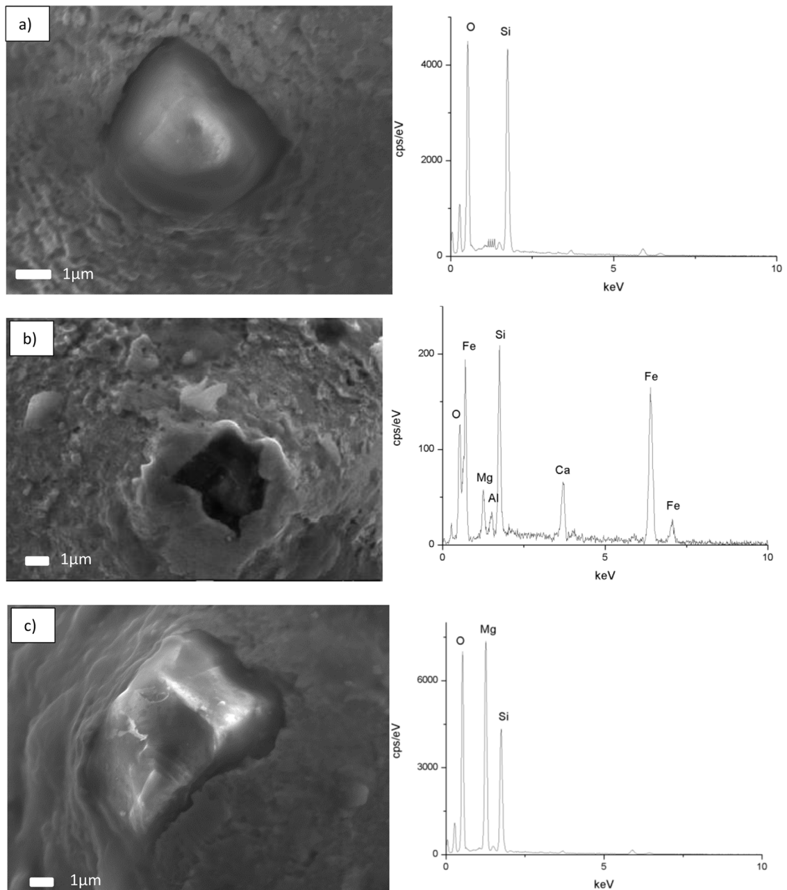
Fig. 2. SEM images and EDS spectra of typical inclusions found on fracture surfaces. a) SiO 2 ; b) SiO 2 -CaO; c) SiO 2 -MgO.
