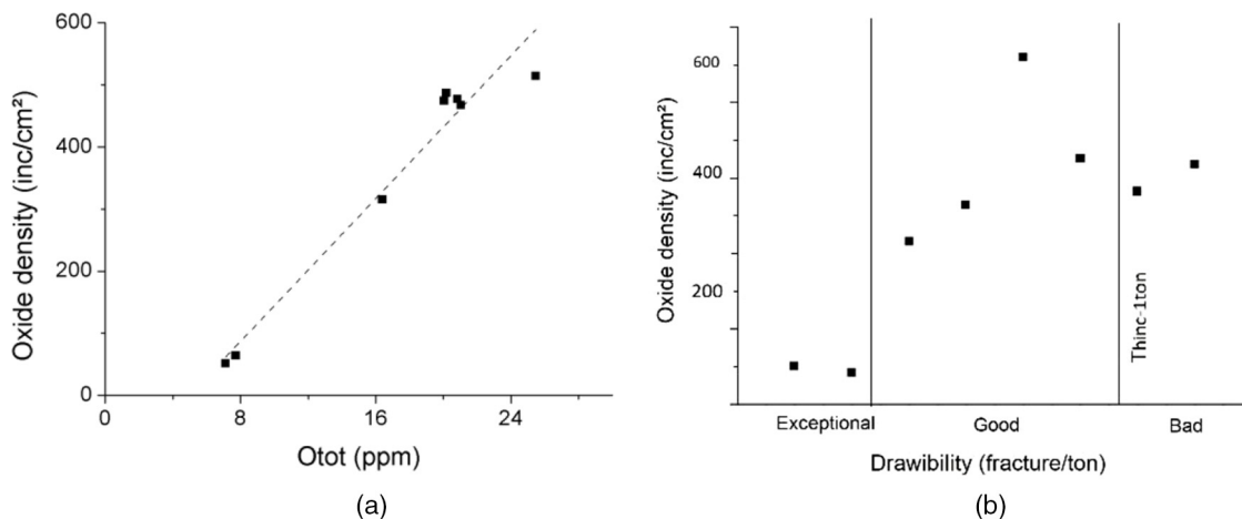
Fig. 7. a) Relation between O_{tot} and oxide density; b) Effect of oxide density on drawability.
