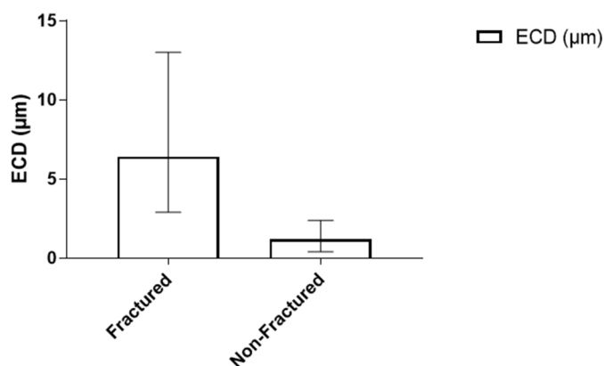
Fig. 8. Effect of the inclusion size on fracture occurrence of wires.
