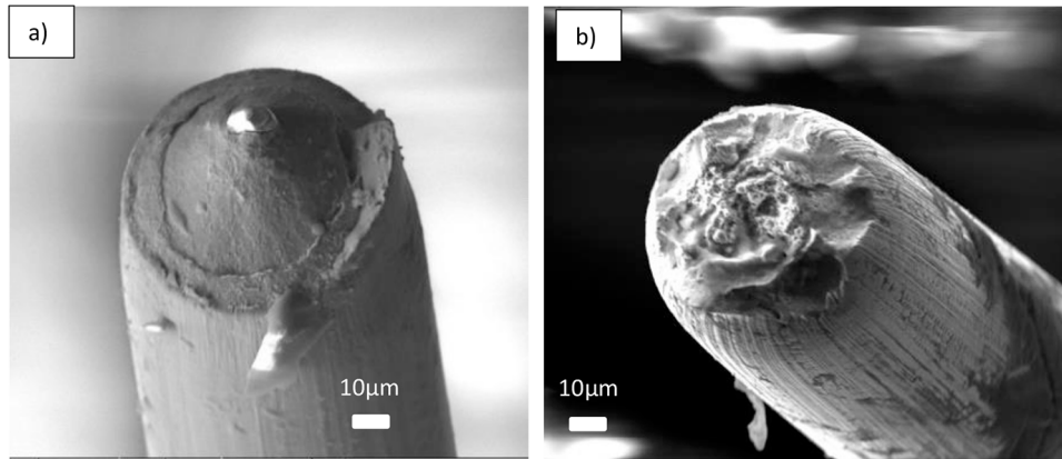
Fig. 1. Fracture surfaces of filaments a) containing an inclusion, b) free of inclusion.
